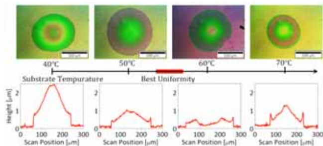
Figure 1. Profiliometry of PZT sol-gel drops printed at different temperatures on a PZT substrate. This result indicates an optimum deposition temperature of approximately 55°C.
